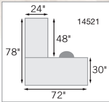
Executive L-Desk
