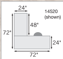
Standard L-Desk
