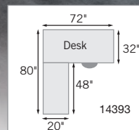
Reversible return
